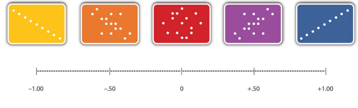
Figure 2.4 Range of Pearson’s r , From -1.00 (Strongest Possible Negative Relationship), Through 0 (No Relationship), to +1.00 (Strongest Possible Positive Relationship)
